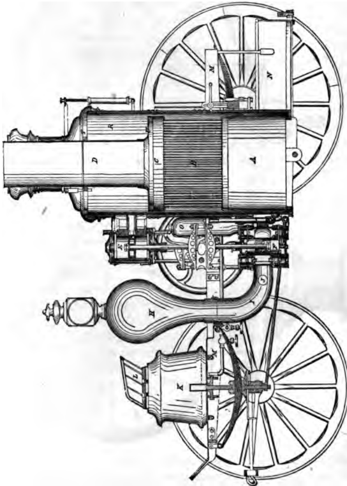
Fig. 131.—The Amokeag Engine. Section.
